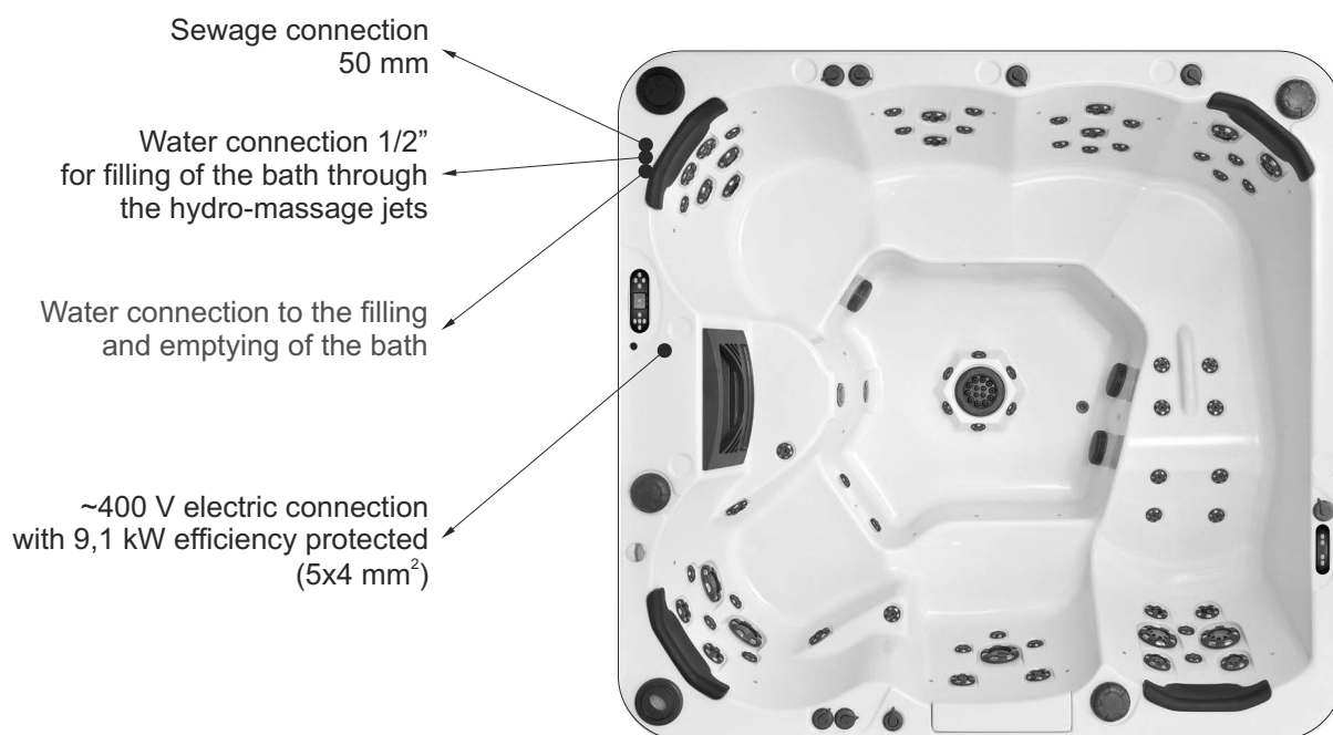
Location of SPA Watrespace connections
