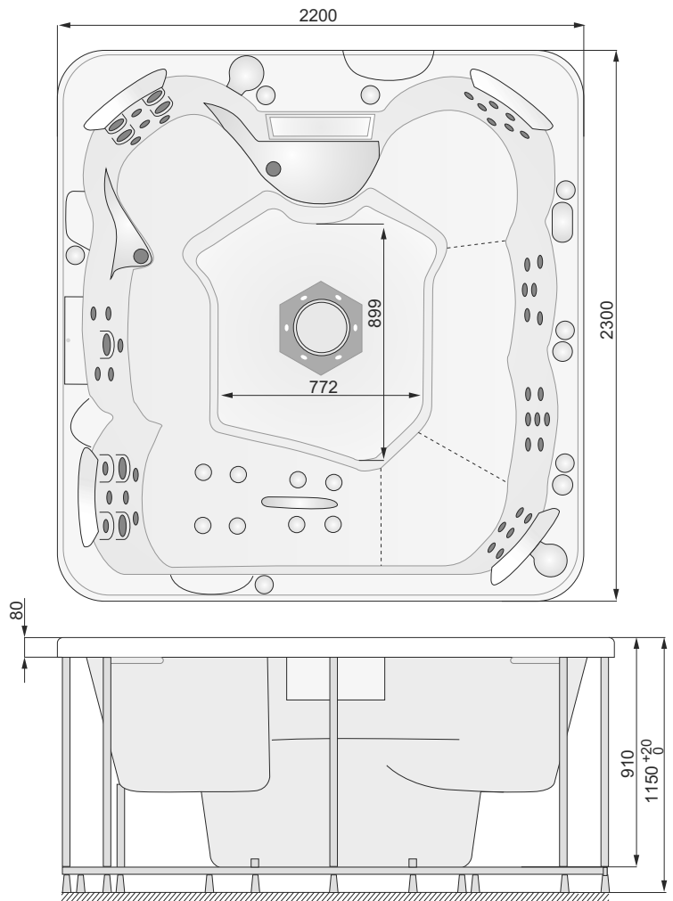
SPA Waterspace dimensions
