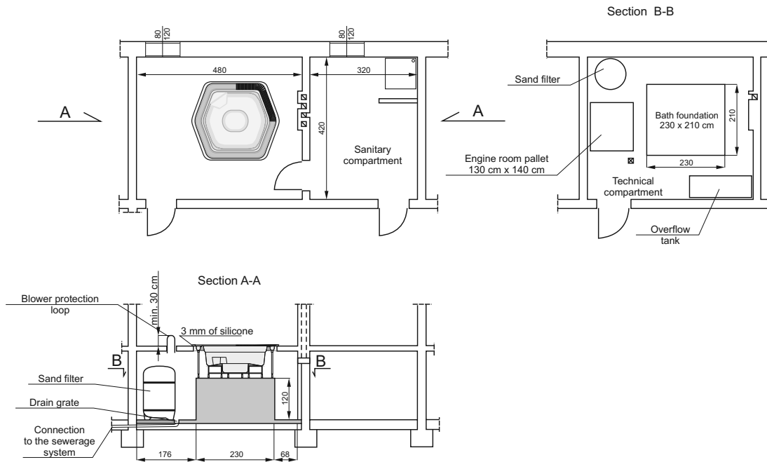
Fig. 2. Bath installed on top of the floor slab
