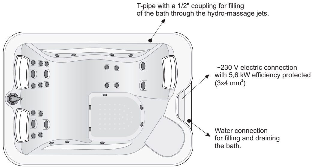
Marina SPA connections
