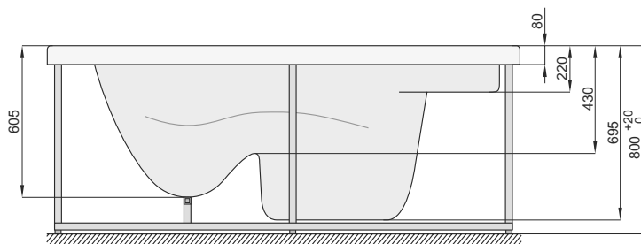
Bath dimensions (aluminium frame)
