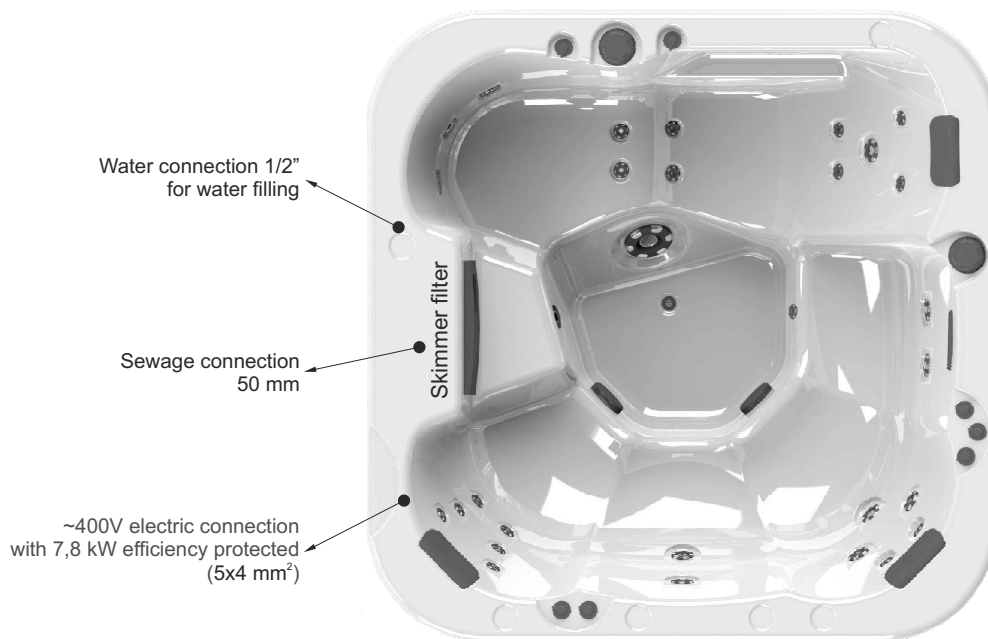
Location of SPA Laguna connections
