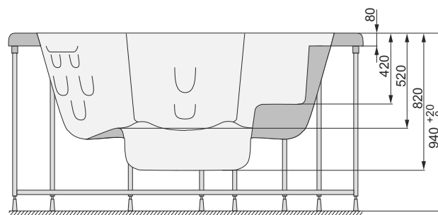
SPA Laguna dimensions
