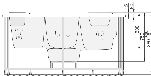
Dimensions of the SPA Katalina bath
