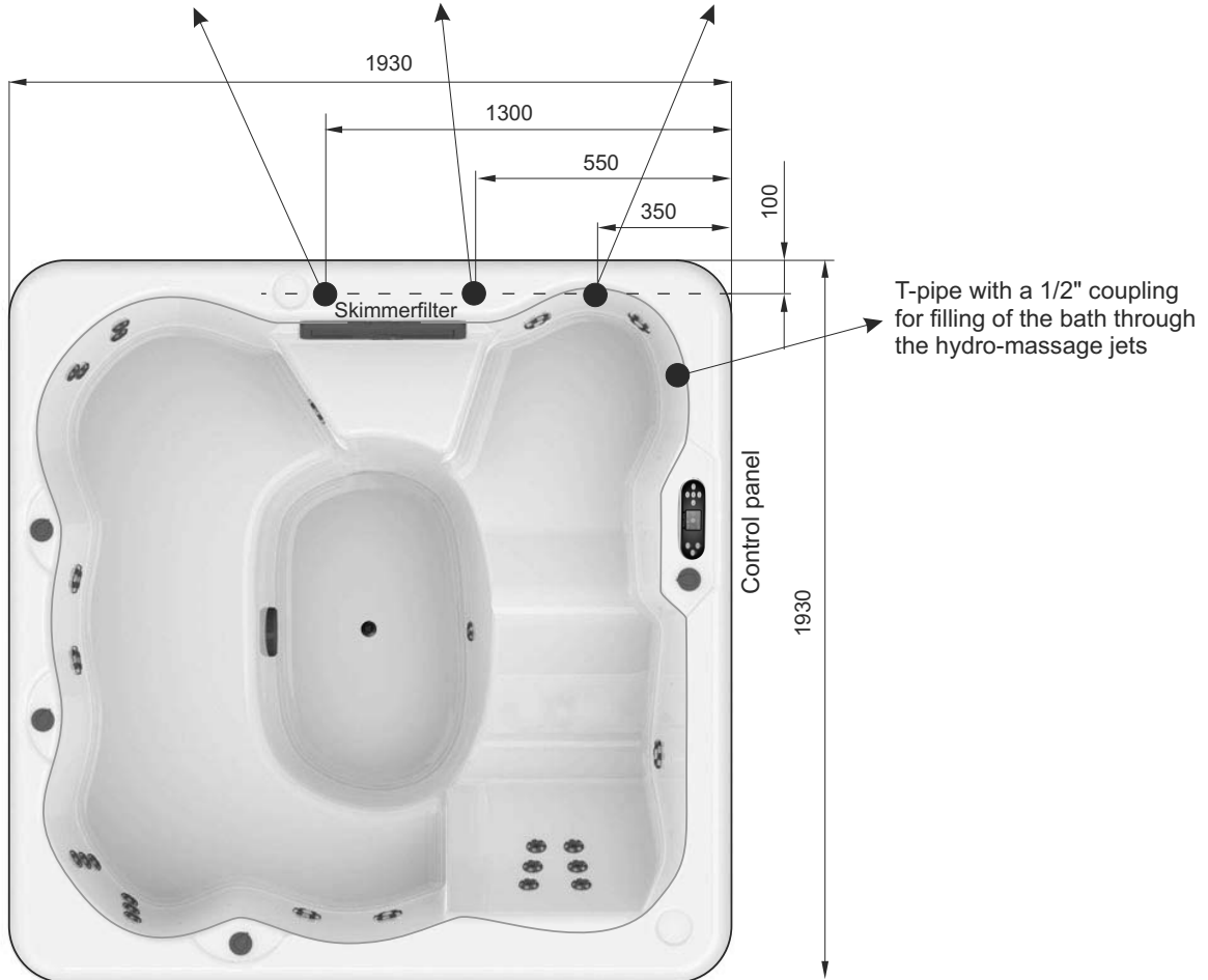
Katalina SPA connections
